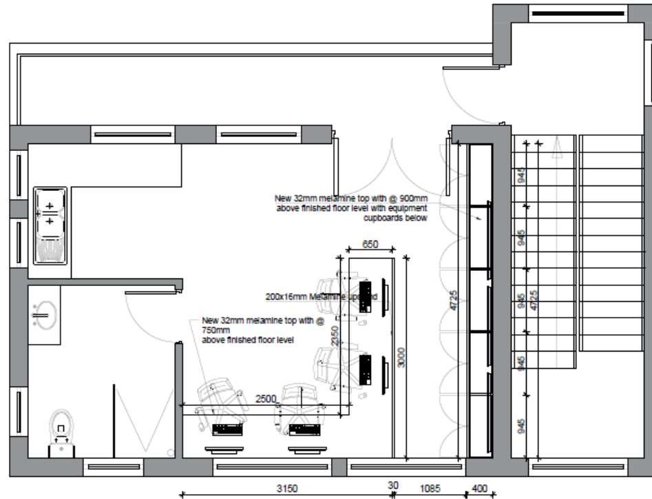
PLAN scale 1:50
