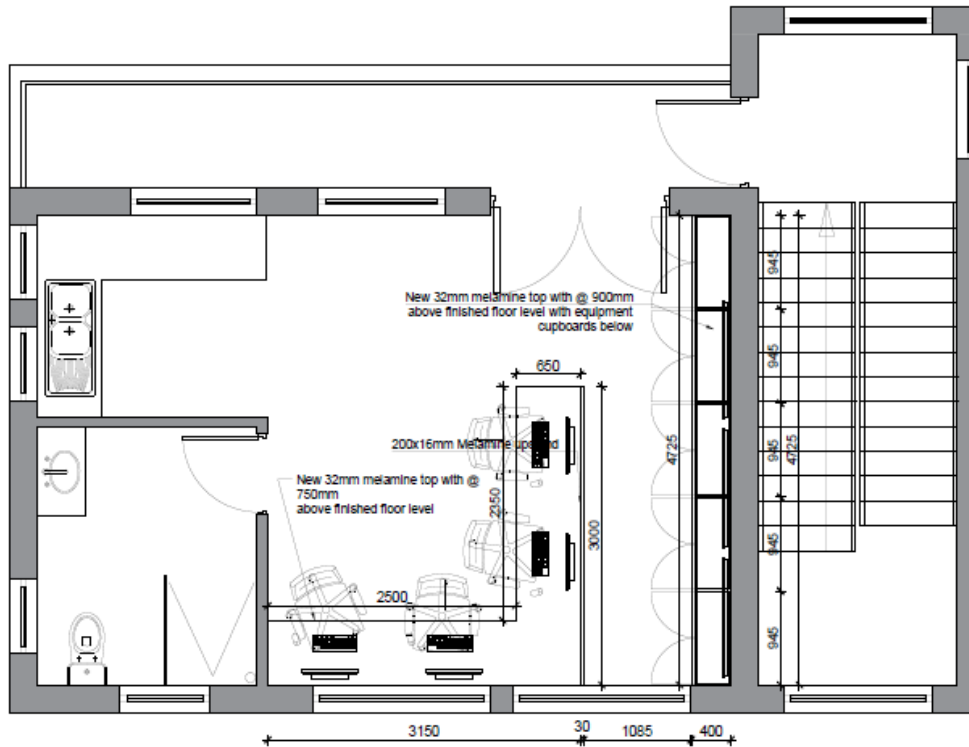
PLAN scale 1:50
