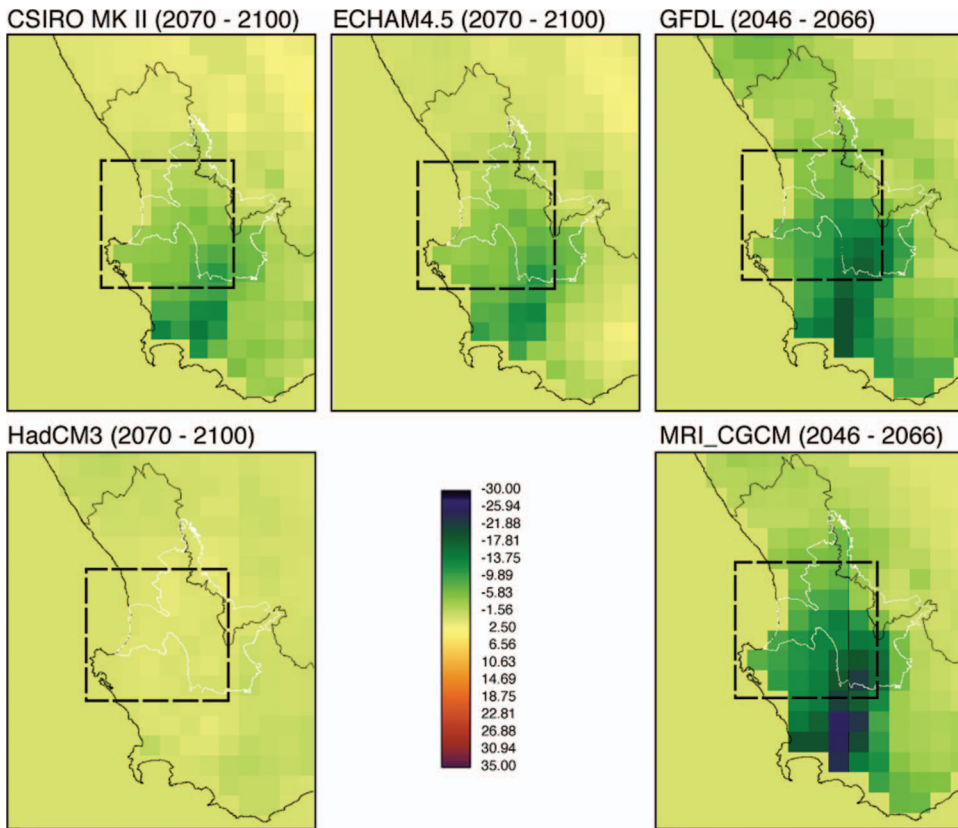
Figure 7. Downscaled winter rainfall anomalies for May–August.
