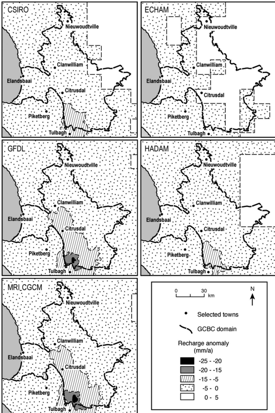
Figure 9. Groundwater recharge depth calculated based on rainfall anomaly using (a) CSIRO model, (b) ECHAM model, (c) GFDL model, (d) HADAM model and (e) MRI_CGCM model.
