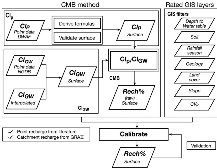
Figure 5. Overview of the recharge calculation process used in the GRAII project (DWAF 2005).
