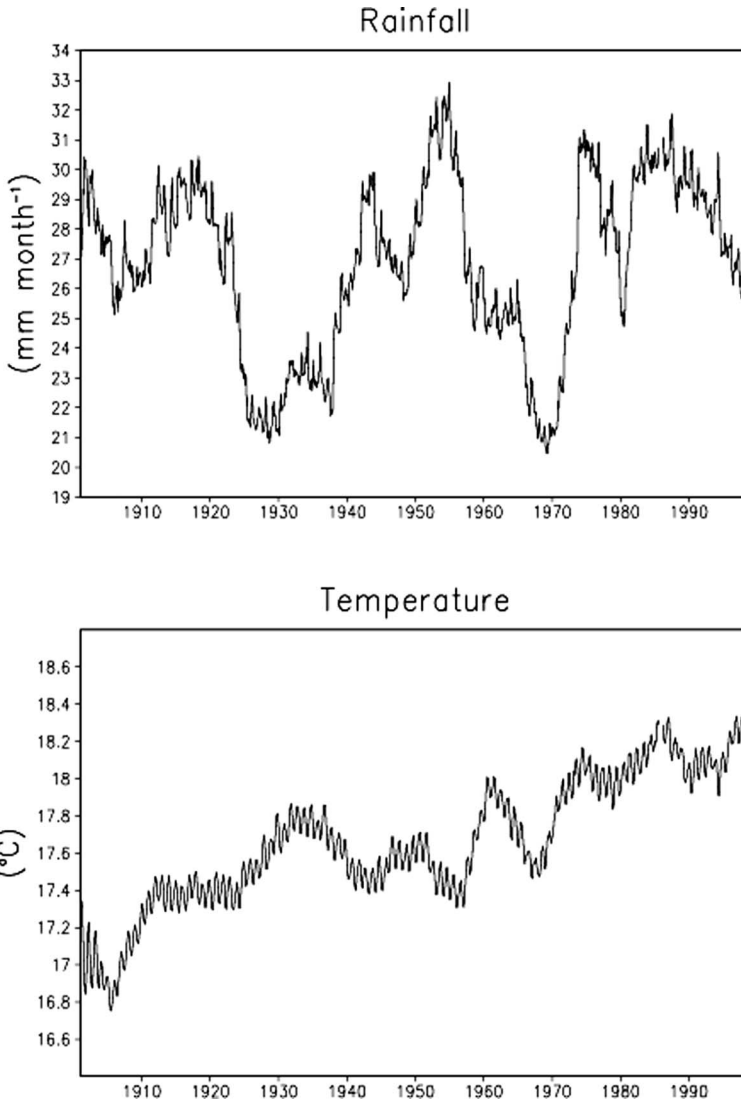
Figure 3. Monthly rainfall and temperature (6 year mean filter) for the Sandveld (1900–1998).
