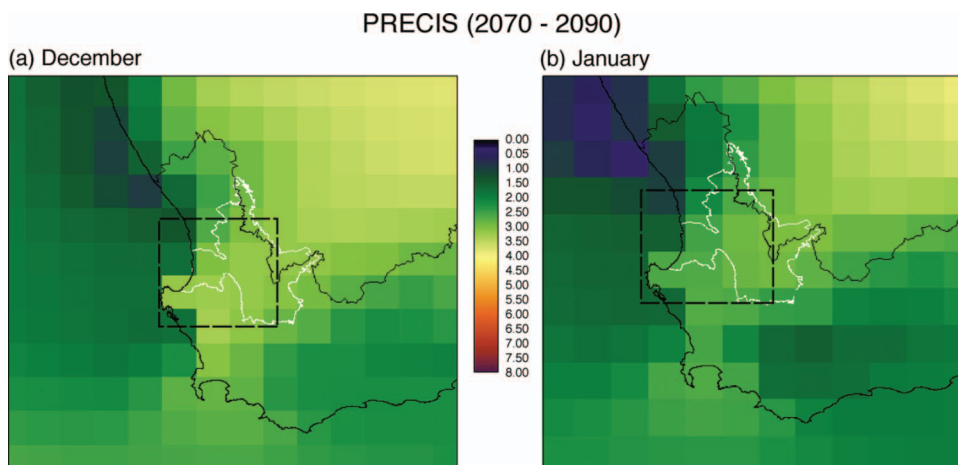
Figure 8. Average maximum temperature anomaly – December and January.
