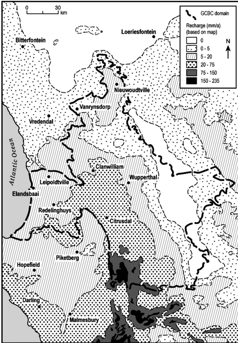
Figure 6. Recharge depth (mm/annum).
