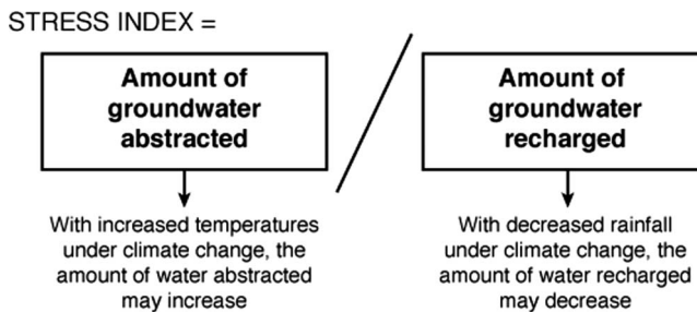
Figure 4. Conceptual model of groundwater stress interaction with climate change.
